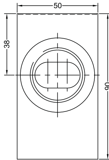
3 PORT 1" BSP-P LINE BODY
