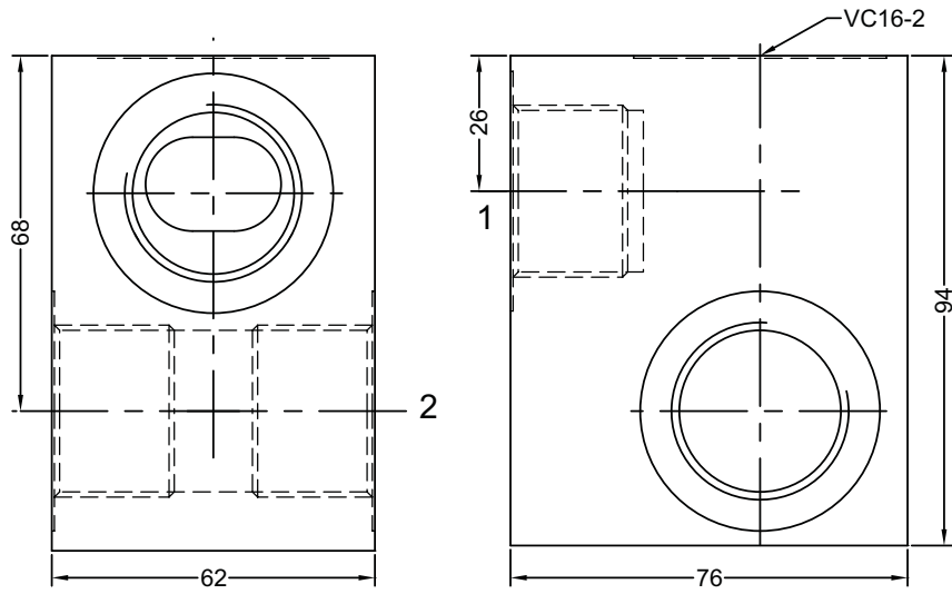
2 PORT 3 WAY 1" BSP-P LINE BODY
