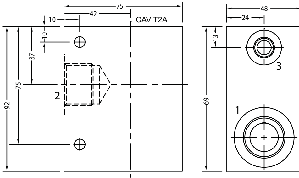
3 PORT 3/4" BSP-P LINE BODY
